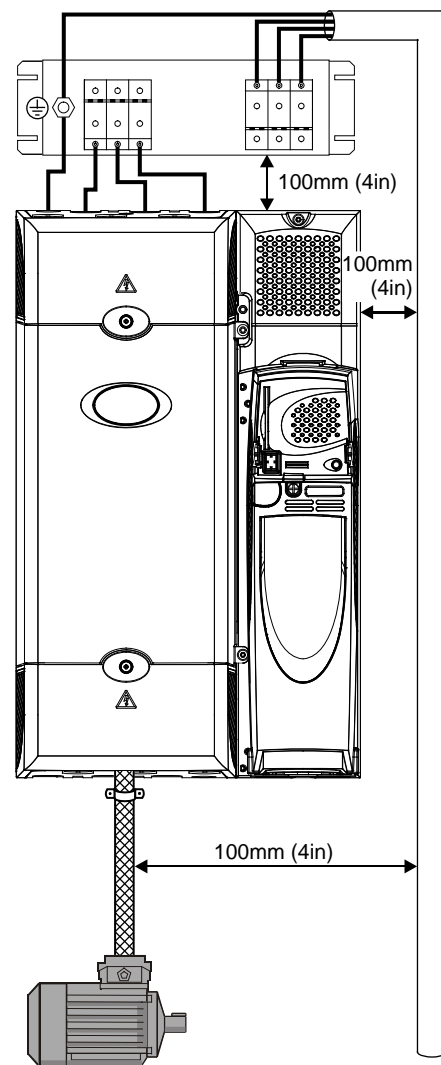
Figure 4: Input wiring spacing
