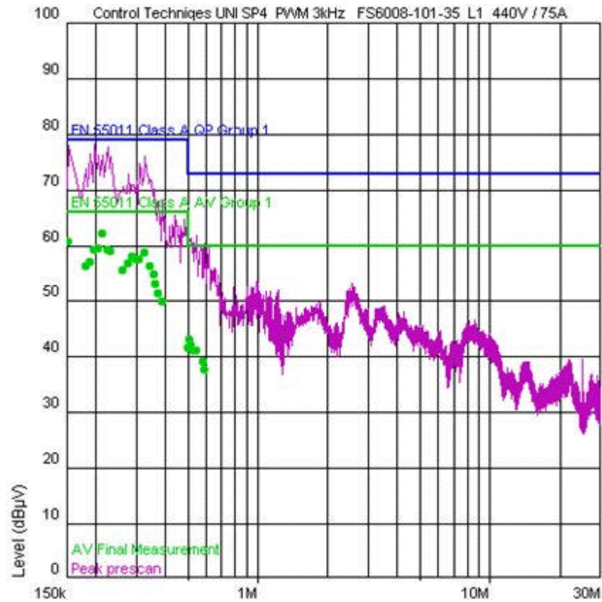
Figure 11: Example conducted emission plot (4403, 100m cable, 3kHz switching frequency)
